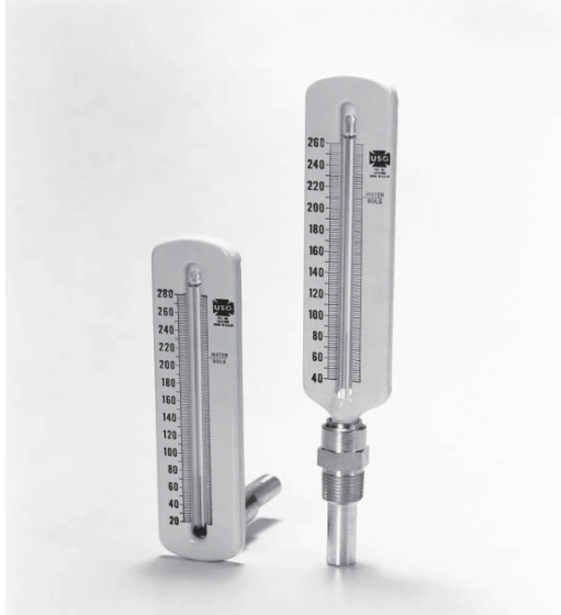
Figure 1: 5" Model T-572 and T-571 (left to right)
