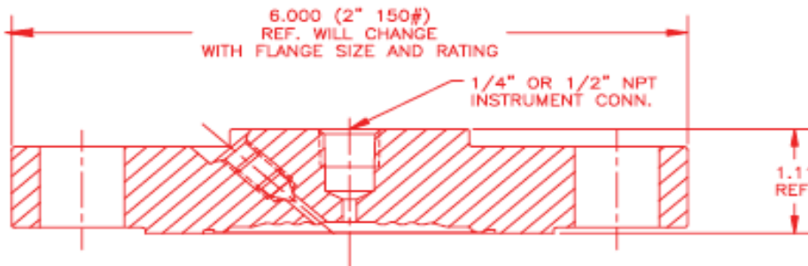
TYPE SFX 2" THRU 4" 150# - 2500# MAX. PRESSURE: 2500 PSI @ 100°F
